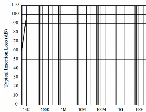
Frequency (Hz) Asymmetric Performance in 50 ohm System With or Without load
